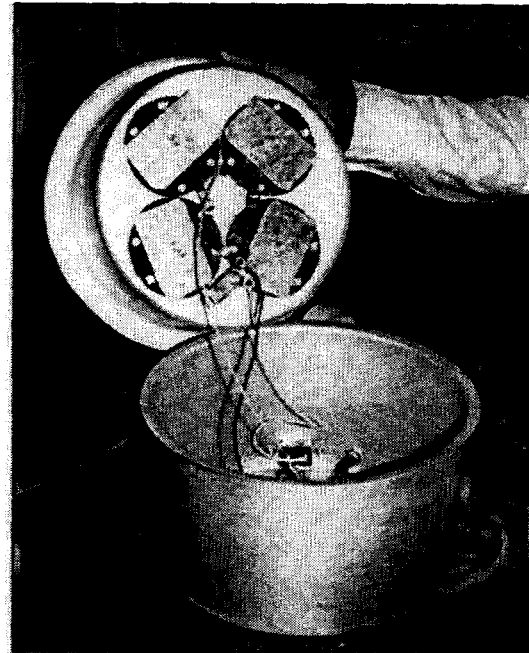
Fig. 14. At the left, a locally manufactured low-wattage cooker in use in a restaurant in Nepal. Above are visible the two sections of the cooker just before their lips are welded together. Four heating elements are installed beneath the inner pot. The socket and pilot light are near the bottom of the outer pot. (Photo credit, below: Lionel Mackay)
