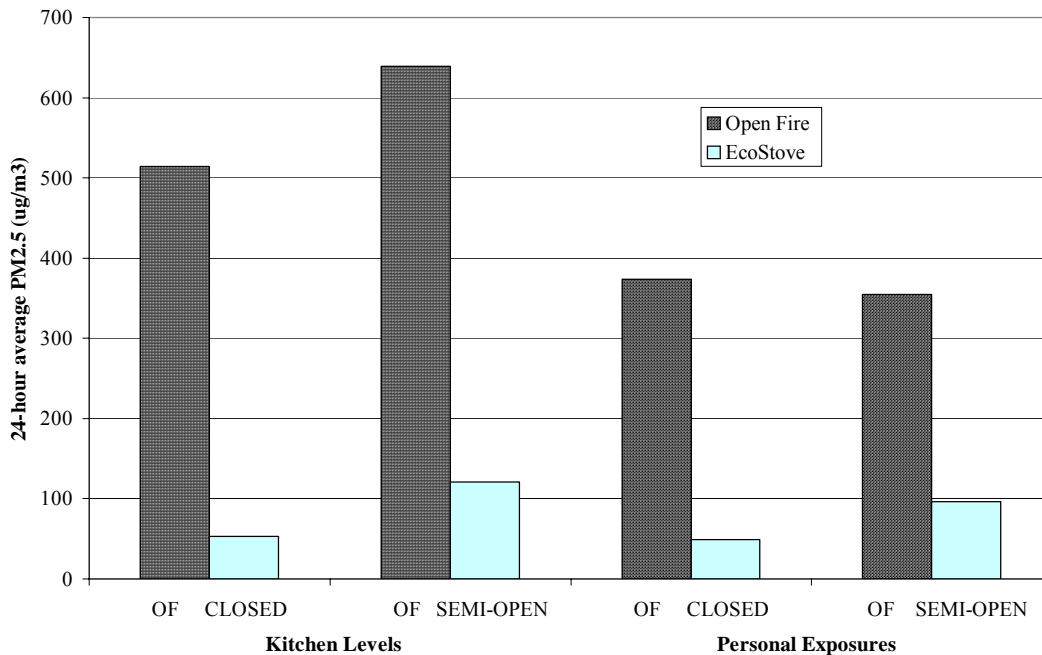
Figure A.2: IAP Levels with the Closed and Semi-Open EcoStoves compared to the Open Fire (OF)
